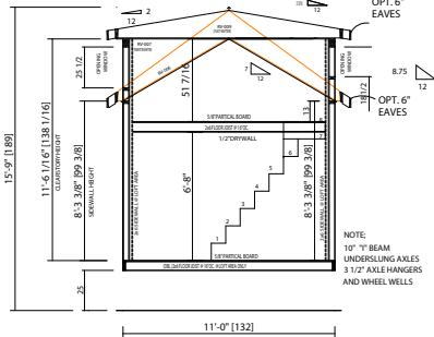
409L CROSS SECTION
