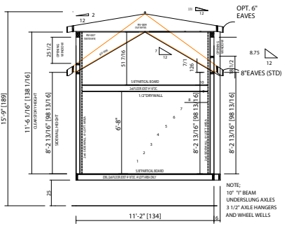
163L CROSS SECTION
